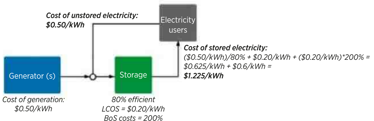
Figure B.3: Simplified diagram demonstrating the costs of storage, neglecting transmission and distribution costs
