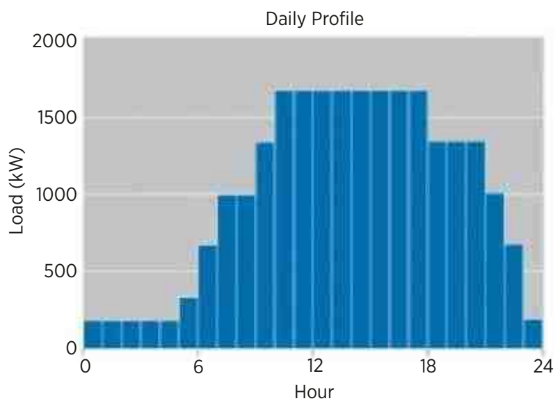
Figure 6: Assumed daily load shape
